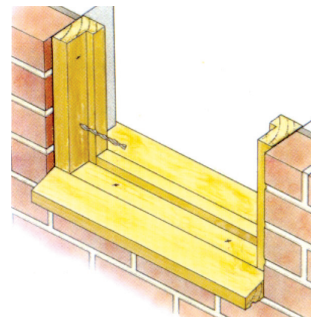
Fixing window and door frames to bricks and blocks
