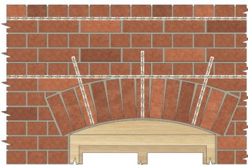
Repairing brick arch lintels
